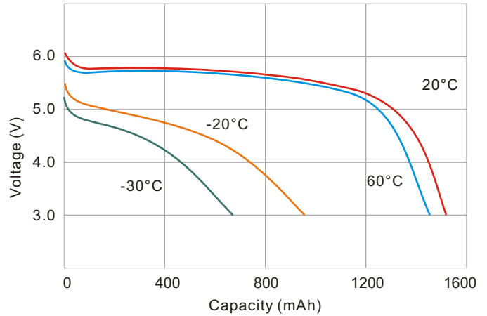
Temperature Characteristics (100mAh)
